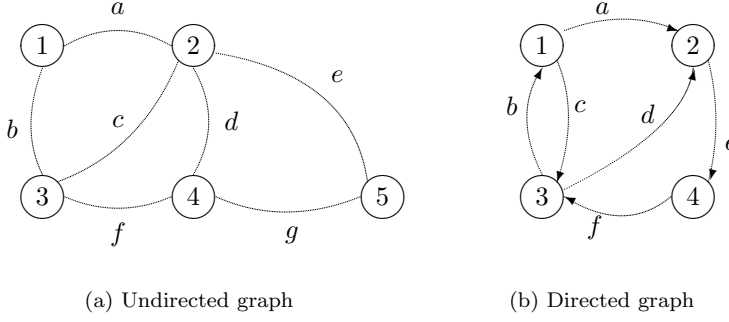
Figure 7.5: Graph representation
